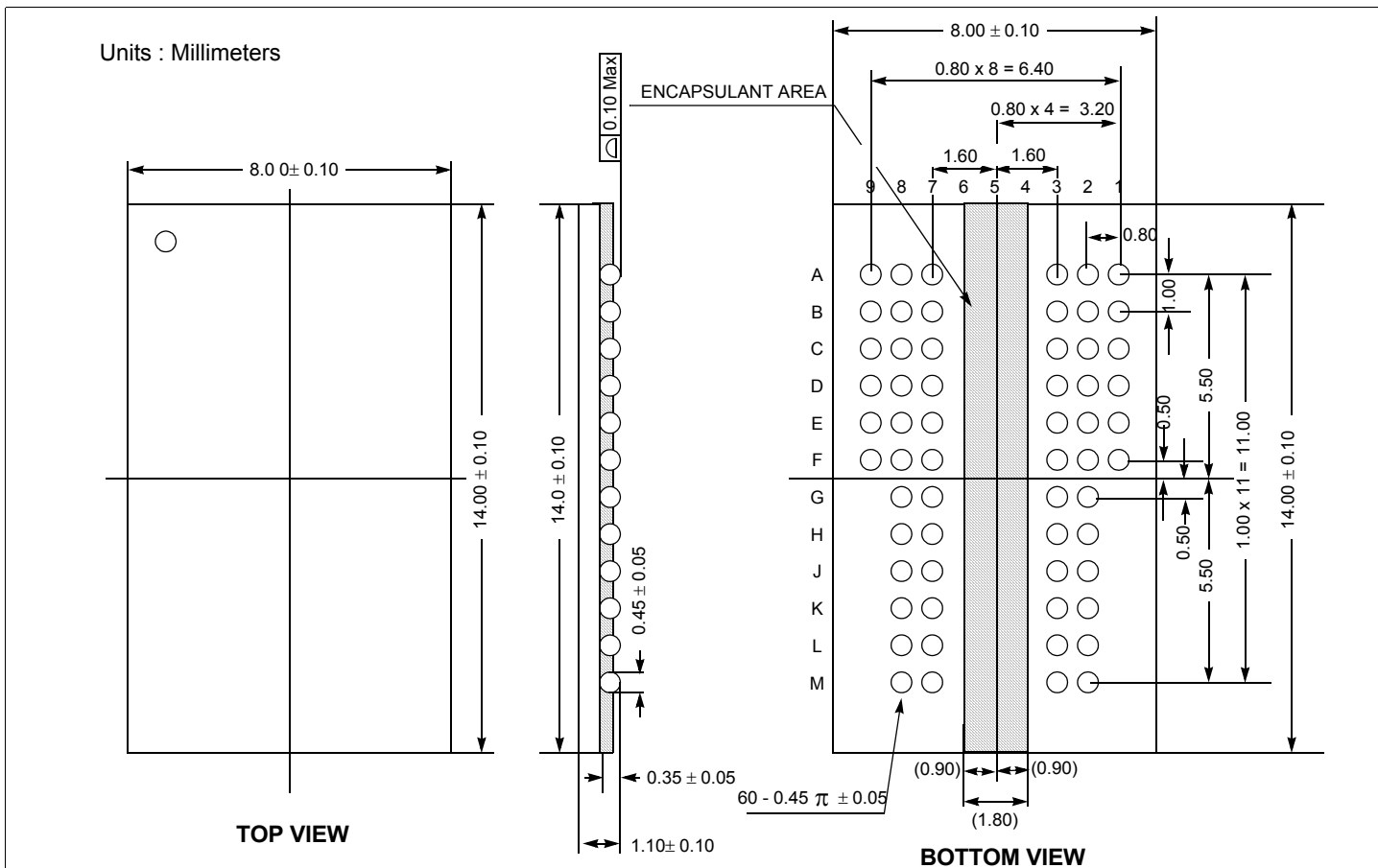
60Ball FBGA Package Dimension
